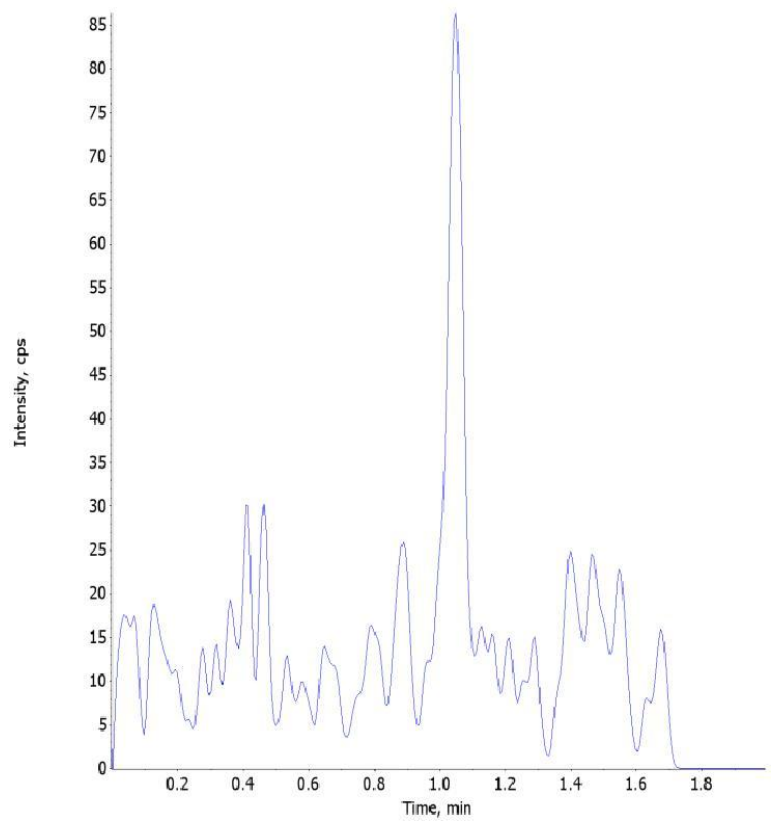
Figure 41: Candesartan zero chromatogram.
